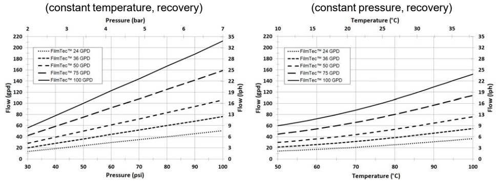
Figure 1: Impact of Pressure on Target Permeate Flow Figure 2: Impact of Temperature on Target Permeate Flow (constant temperature, recovery) (constant pressure, recovery)
