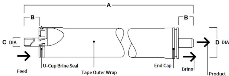
FilmTec™ coupler part number 89055 is ordered separately for each element. Each coupler includes two 2.230 EPR O-rings (part number 89250).
