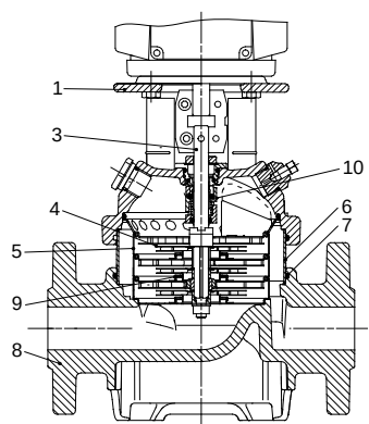
Sectional drawing
