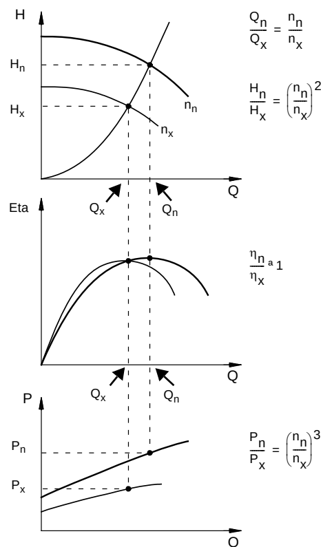
Fig. 13 Affinity equations
