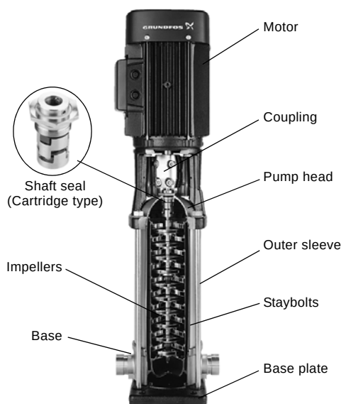
Fig. 2 CR pump
