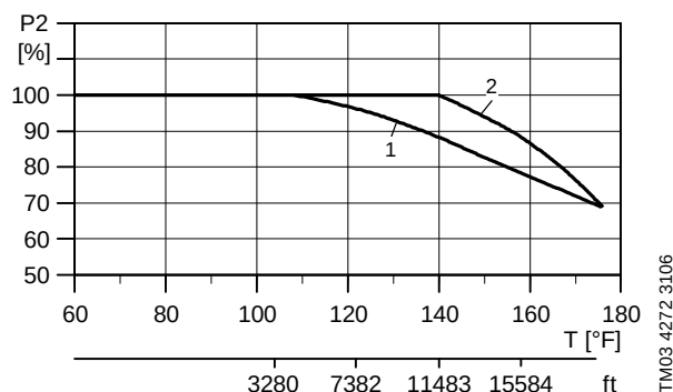
Fig. 4 Relationship between motor output ( P_2 ) and ambient temperature/altitude
