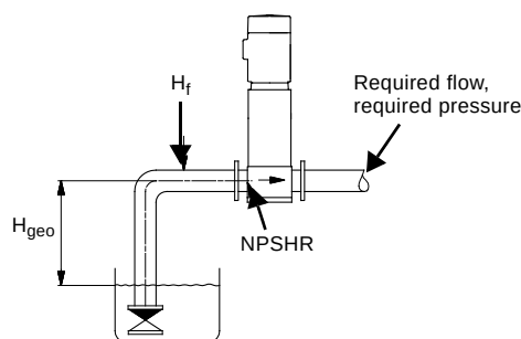
Fig. 9 Sizing data
